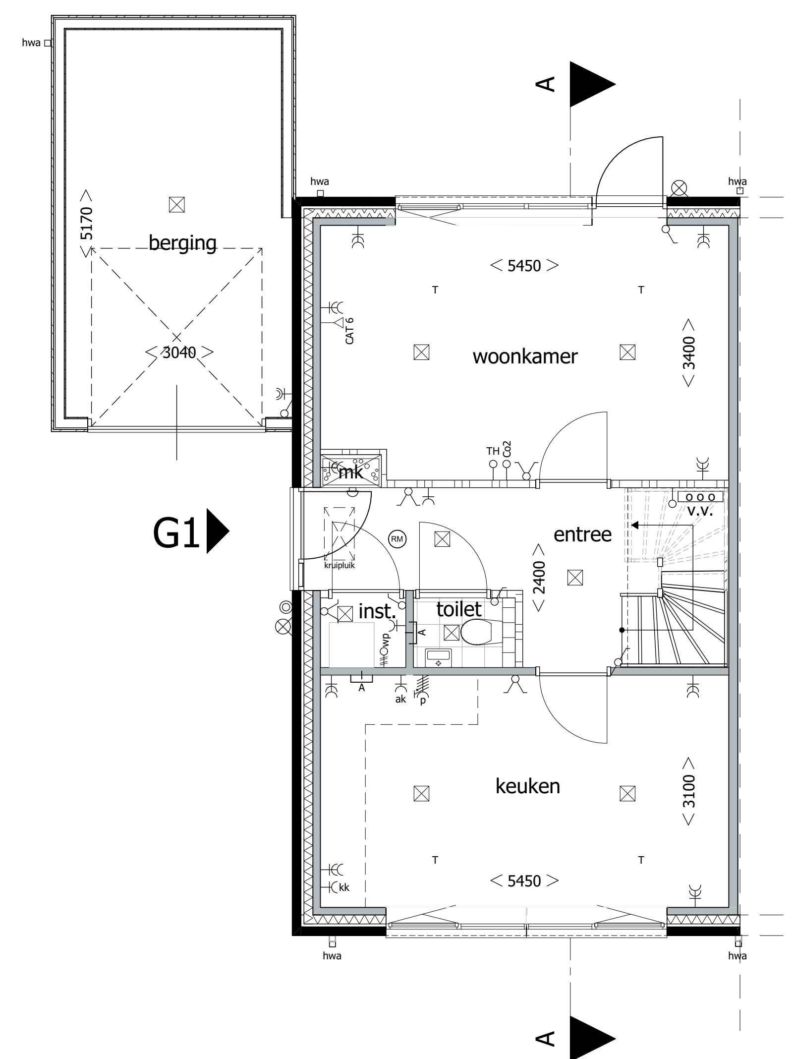
Begane grond type G1
